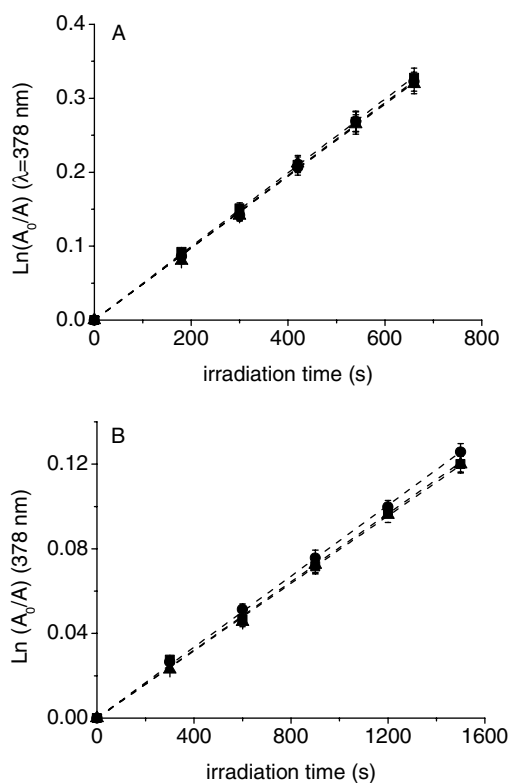
Figure 2. First-order plots for the photooxidation of (A) DMA ( 30 \mu\text{M} ) and (B) DMA ( 30 \mu\text{M} ) in the presence of Car ( 12 \mu\text{M} ) by ZnPc 3 (■), ZnPc 4 (●) and ZnPc (▲), in THF, \lambda_{\text{irr}} = 675 \text{ nm} . Values represent mean \pm standard deviation.
