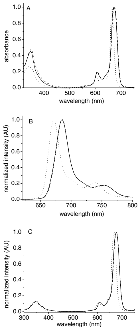
Figure 1. (A) Absorption spectra; (B) fluorescence emission spectra ( \lambda_{\text{exc}} = 608 \text{ nm} ) and (C) fluorescence excitation spectra ( \lambda_{\text{em}} = 740 \text{ nm} ) of ZnPc 3 (solid line), ZnPc 4 (dashed line) and ZnPc (dotted line) in THF.
