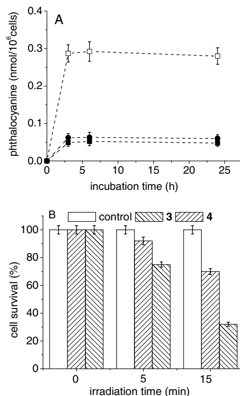
Figure 3. (A) Uptake of ZnPc 3 (■) 0.1 \mu\text{M} , ZnPc 3 (□) 0.5 \mu\text{M} and ZnPc 4 (●) 0.1 \mu\text{M} into Hep-2 cells as a function of incubation time; (B) inactivation of Hep-2 cells treated with phthalocyanine and exposed to different irradiation times with visible light; [phthalocyanine] = 0.1 \mu\text{M} ; incubation time 24h. Values represent mean \pm standard deviation of three separate experiments.
