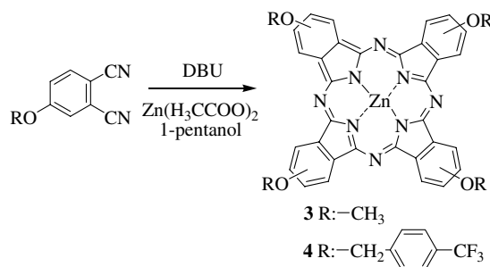
Scheme 2. Synthesis of phthalocyanine derivatives.
